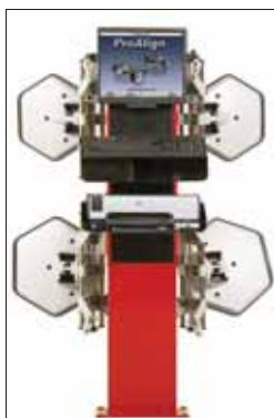
20-2313-1 Alternative Mounting Base
